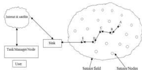
Figure 1: Communication architecture of wireless sensor networks
