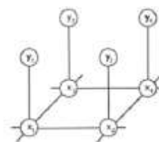
Fig. 2: RF Model : x_k – unknown HR patches;
