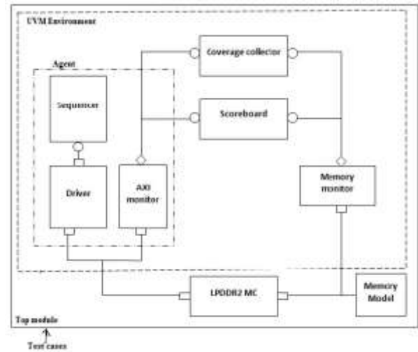
Figure.4 coverage collector in UVM environment
