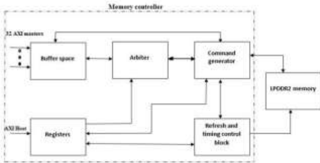
Figure.2 Simplified block diagram of LPDDR2 MC
