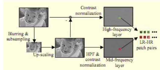
Fig. 5: Preprocessing for dictionary construction
