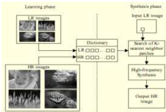
Fig. 4: HR-LR Dictionary Learning Based SR model.
