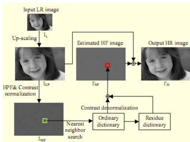
Fig. 7: Synthesis Phase
