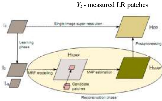
Fig. 3: Learning Based SR model.
