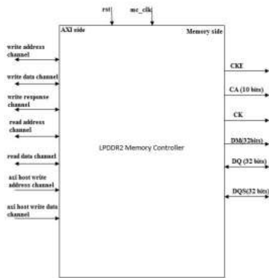
Figure.3 Interfaces of LPDDR2 MC
