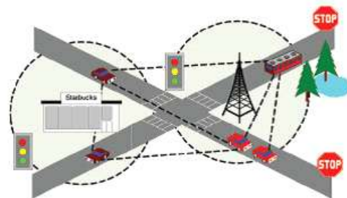
Figure 3 Hybrid Architecture
