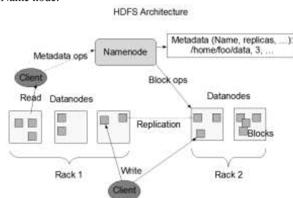
Fig 4: HDFS Architecture
