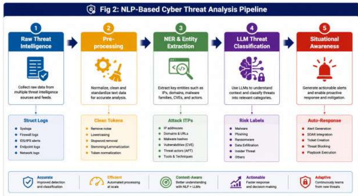
Fig. 2: NLP-Based Cyber Threat Analysis Pipeline. Five sequential stages transform raw threat intelligence into structured situational awareness outputs and automated remediation triggers.
