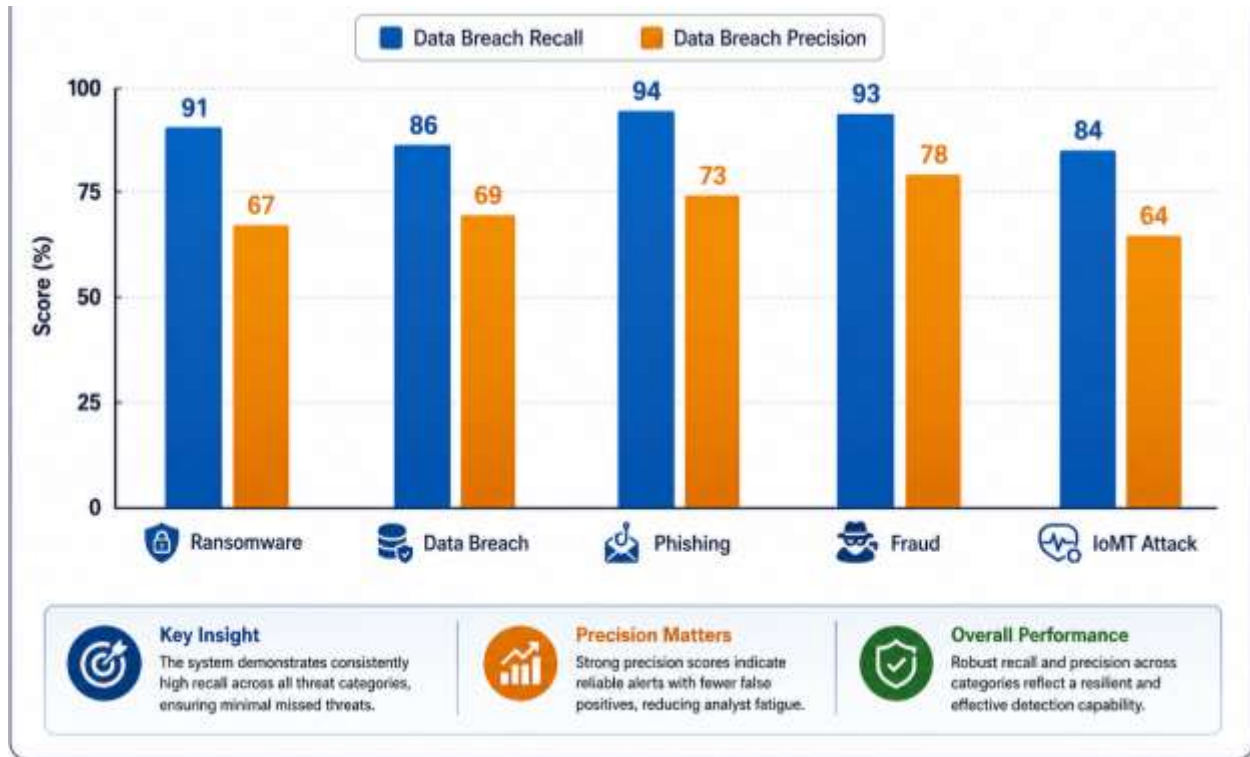
Fig. 4: SHCDF Performance by Threat Category. Recall (blue) consistently exceeds 84% across all categories; precision (amber) ranges from 64% to 78%, reflecting the domain-specific challenge of false-positive reduction in heterogeneous data environments.
