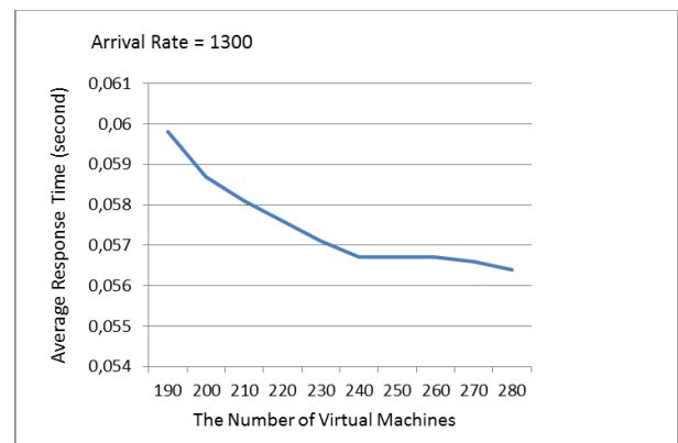
Figure. 3 The average response system time in every number of Virtual Machines for the number of arrival rate 1300
